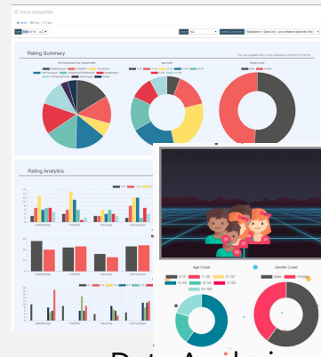
Data Analysis
